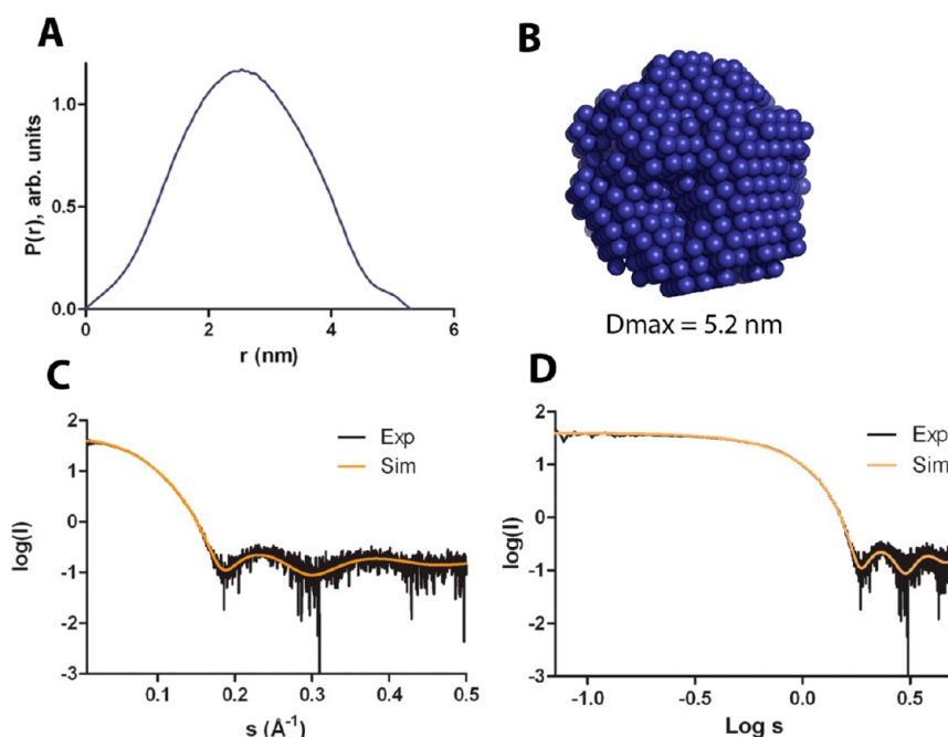
Figure 6. SAXS of IDeg in the presence of zinc, imidazole, and resorcinol. SAXS scattering data of IDeg (0.2–1.4 mM) containing 3 \text{Zn}^{2+} /6Ins, 20 mM resorcinol, 100 mM imidazole, 100 mM NaCl, and 10 mM Tris (pH 7.5). (A) Data presented as the pair distance distribution function collected from a sample. (B) An ab initio model calculated by DAMMIF. The spherical character and dimensions of the model resemble those of an insulin hexamer. (C and D) When the hexamer crystal structure was applied for simulation of scattering curves (orange), a very good fit in the high-resolution (C) and low-resolution (D) regions was obtained when compared with the experimental data (black).
