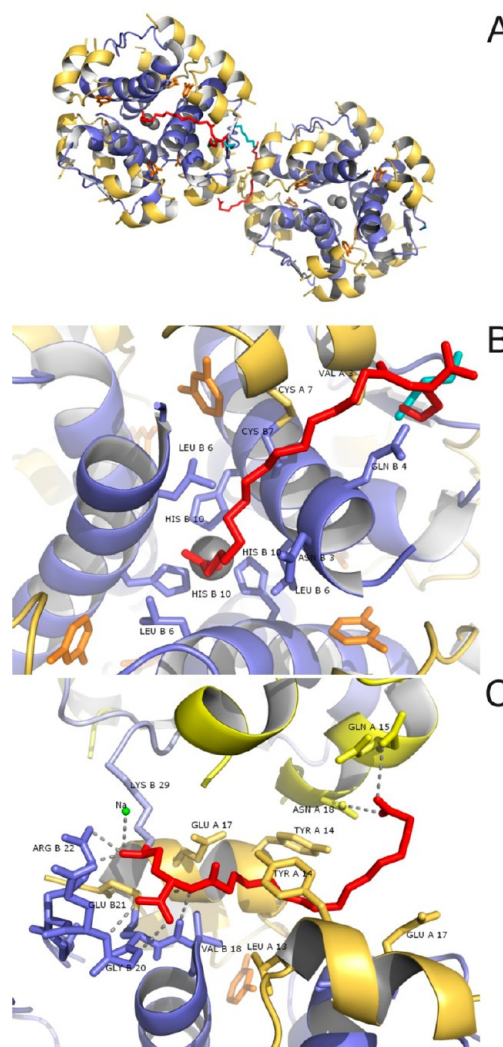
Figure 2. Crystal structure of IDeg in complex with zinc and phenolic ligands. (A) Location of the B29-linked fatty diacid on the IDeg hexamer in the monoclinic crystal involving a neighboring insulin hexamer in the crystal. The two neighboring insulin hexamers are drawn as cartoons with A-chains colored yellow and B-chains blue. Zinc is depicted as gray spheres, and resorcinol molecules are colored orange. The fatty diacid moieties are colored red, and the Lys B29 side chain to which the fatty diacids are covalently attached is colored cyan. (B) Fatty diacid 1, the fatty diacid moiety that coordinates to the structural zinc atom. Side chains that are in the vicinity of 3.5 Å of the fatty diacid are depicted as sticks. The coloring is similar to that of panel A. (C) Fatty diacid 2, which is common for the rhombohedral form. The monoclinic crystal binds to a hydrophobic area on a neighboring hexamer. Side chains within 3.5 Å of the fatty diacid are shown as sticks. Hydrogen bonds or polar contacts are indicated as dashed lines.
