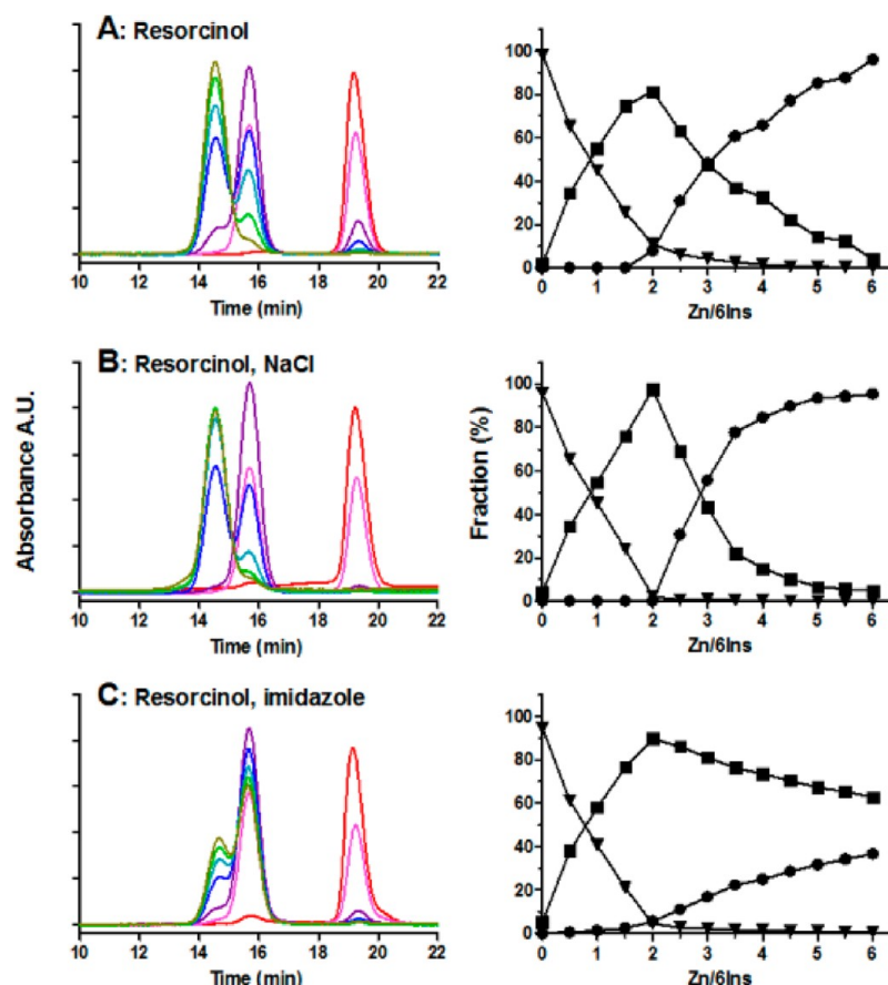
Figure 5. Size distribution of IDEg in the presence of \text{Zn}^{2+} , resorcinol, NaCl, and imidazole. Chromatograms (left) and species distribution (right) of IDEg in the presence of \text{Zn}^{2+} , resorcinol, NaCl, and imidazole. The zinc ratios varied in integers from 0–6 \text{Zn}^{2+}/6\text{Ins} and are depicted in various colors (red, pink, purple, blue, cyan, green, and olive), and the species distribution obtained from the SEC after integration is indicated by triangles (monomer), squares (presumed hexamer), and circles (dihexamer). The molecular mass standards (not shown) were similar to those depicted in Figure 3. (A) Samples of 0.6 mM IDEg and 30 mM resorcinol (pH 7.4). (B) Samples of 0.6 mM IDEg, 150 mM NaCl, and 30 mM resorcinol (pH 7.4). (C) Samples of 0.6 mM IDEg, 100 mM imidazole, and 30 mM resorcinol (pH 7.4).
