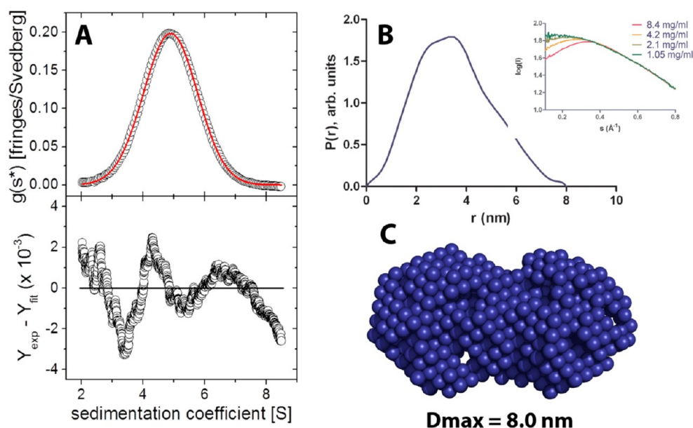
Figure 4. AUC and SAXS of IDeg in the presence of zinc and phenol. (A) AUC of 0.19 \mu\text{M} IDeg, 5 \text{Zn}^{2+} /6Ins, and 30 mM phenol (pH 7.4) depicted as a g(s^*) curve (top, open circles); only every 10th data point is shown. The red line represents simulated data for a single sedimenting species with an s of 4.94 S, a D^* of 6.31 \times 10^{-7} \text{ cm}^2/\text{s} , and an M_w of 75.1 kg/mol. The deviations between the experimental and simulated data are displayed (bottom); every data point is shown, with an overall rmsd of 1.19 mFringes. (B) SAXS of IDeg with 5 \text{Zn}^{2+} /6Ins and 5 mM phenol (pH 7.5) depicted as a pair distance distribution plot, P(r) . From the plot, D_{\text{max}} was determined to be 8.0 nm. The inset shows the experimental SAXS data and the concentration-dependent intensity decrease at low values of r , caused by interparticle interference at high concentrations. (C) SAXS model based on the data presented in panel B. The model is an averaged and filtered ab initio bead model calculated with DAMMIF.
